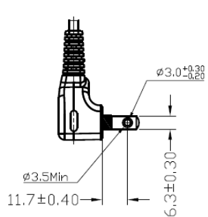
90° Plug view
