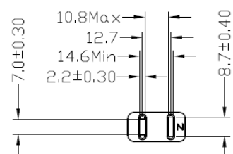
Outlet View
